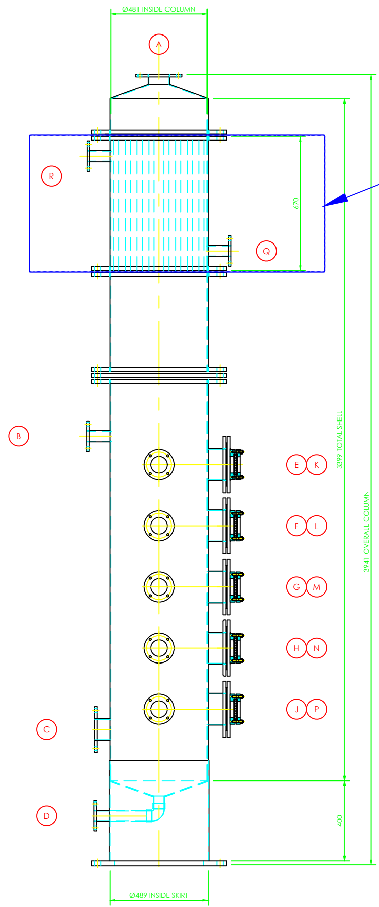
ELEVATION VIEW SEE PLAN VIEW FOR TRUE NOZZLE ORIENTATIONS
